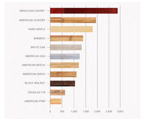
Janka Scale
