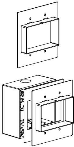
STEALTH PATHLIGHT MOUNTING
