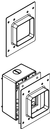
DOUBLE IMPACT MOUNTING PLATE
