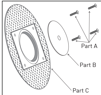
Figure 1. DLA-APP-Z-RD (DLA-APP-Z-SQ equipped with same parts and quantity. Appliqué and plaster plug shape differ.)
